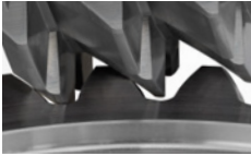
Hobbing and chamfer cutting
